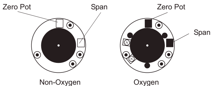
Diagram 15: Sensepoint Toxic Sensor Zero and Span potentiometer
