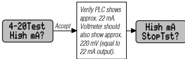
Figure 7. 4/20 Loop Full Scale Test
