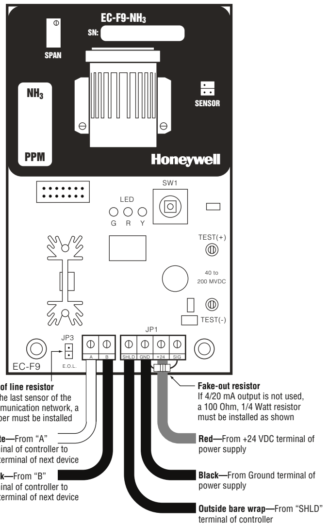
Figure 3. RS-485 Communication and Power Wiring Diagram
