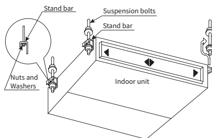
Figure 4.6 Hoisting method
