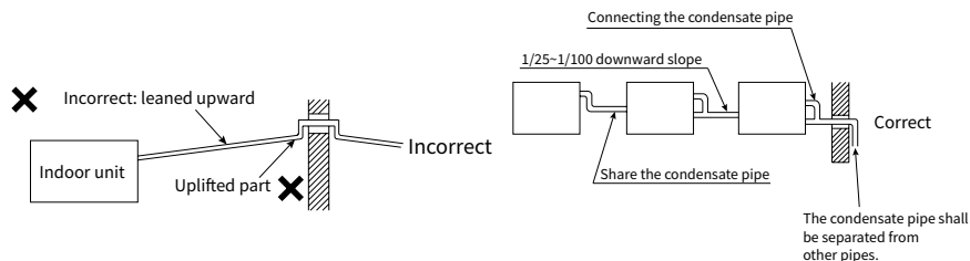
Figure 6.1 Condensate Pipe
