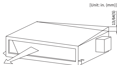
Figure 4.7 Gradient of the Top Surface
