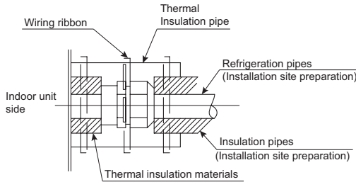
Figure 5.5 Heat Preservation
