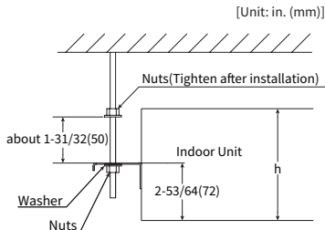
Figure 4.5 Hanging Bolt and Nut
