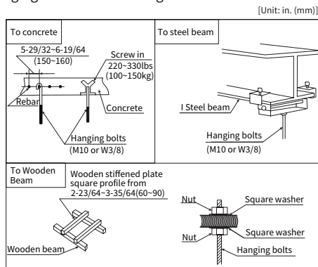
Figure 4.2 Fixation of Hanging Bolts
