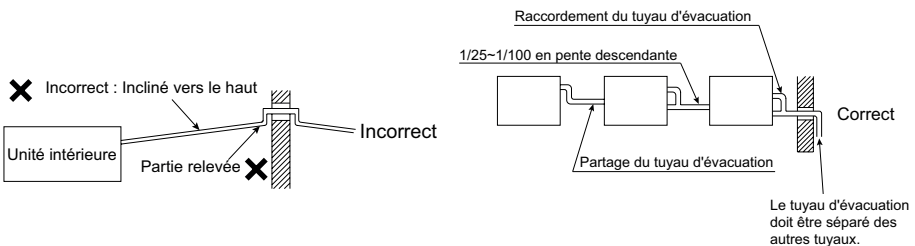
Figure 6.1 Tuyau de condensat
