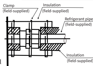
Piping insulation procedure
