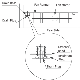
Fig.6.2 Drain Plug
