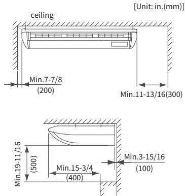
Fig.4.1 Operation and Maintenance Space
