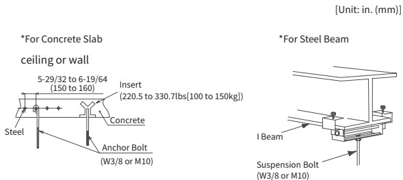
Fig.4.2 Mounting of Suspension Bolts
