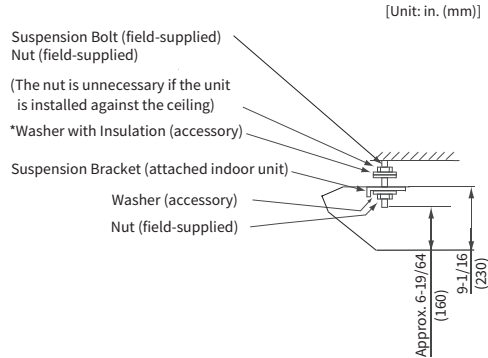
Fig.4.5 Mounting Nuts and Washers
