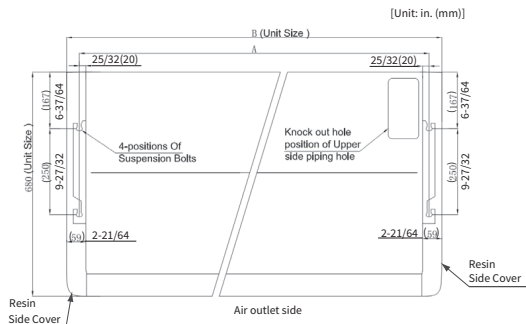
Fig.4.4 Mounting Position
