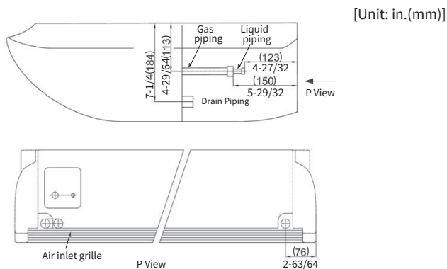
Fig.5.1 Piping Connection of Indoor Unit
