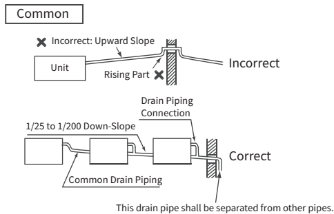
Fig.6.6 Drain Piping
