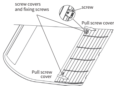
Fig.6.1 Open the air inlet grille
