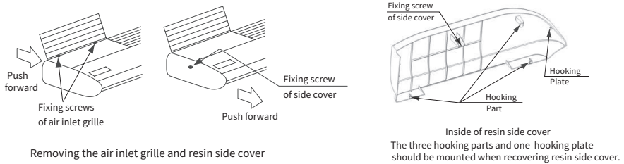
Fig.3.2 Removing the air inlet grille and resin side cover
