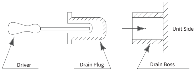
Fig.6.3 Inserting Drain Plug
