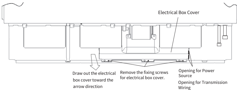
Fig.7.1 Remove electrical box cover
