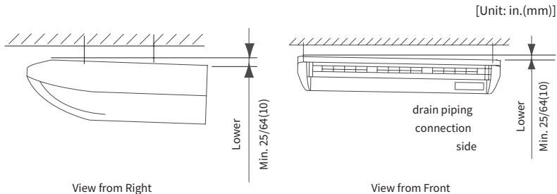
Fig.4.6 Inclination of Unit for Drain for ceiling installation
