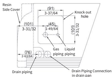
Fig.5.1 Piping Connection of Indoor Unit
